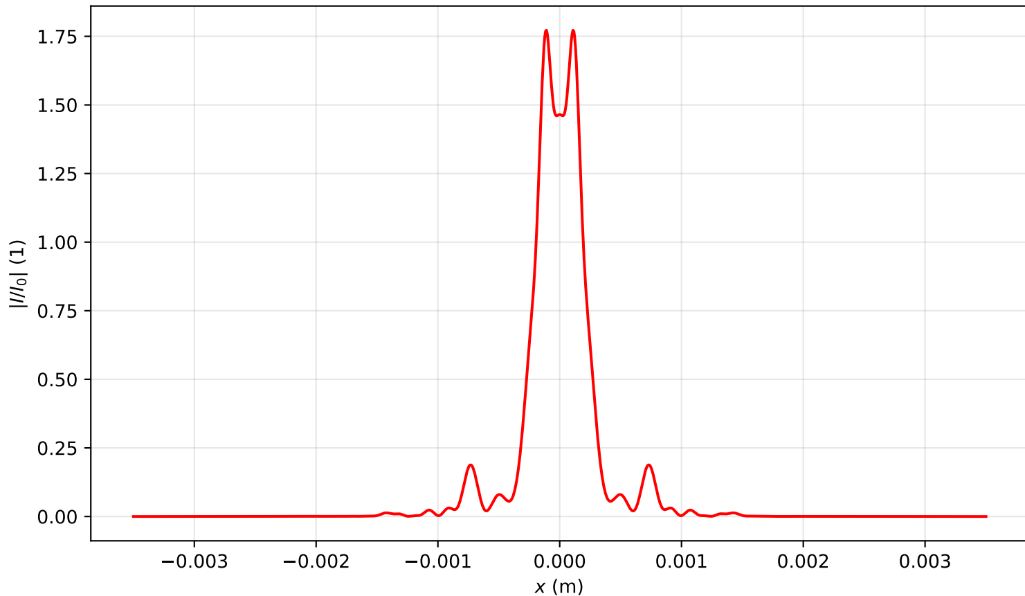
Intensity profile I(x, y = 0, z = 0.955)/I_0 , P_{in}=7.5P_{cr} , artificial time
